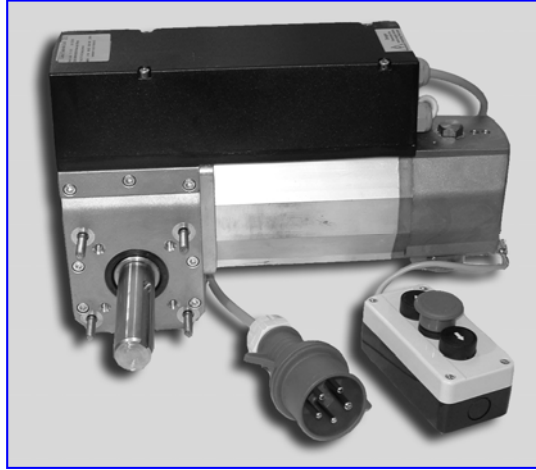
CDO100 EV 1 (BOS) Part # 8050 Shown with 1 1/4 output shaft, built on control panel, pre-wired 3ph plug and push button station .
